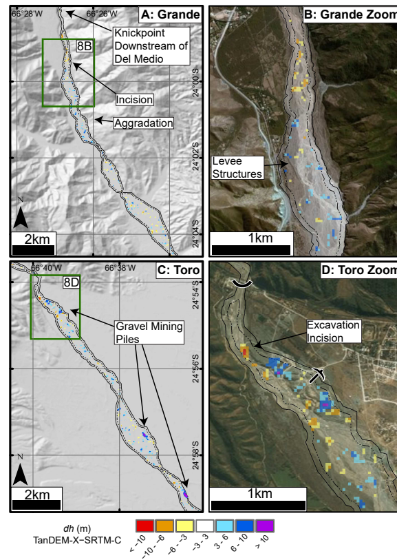
Figure 3.8 – Map-views of the in-channel dh measurements for Río Grande (A) and Río Toro (C) highlighted in the longitudinal profiles in Figure 3.7. For location of each map refer to Figure 3.1C. More details are shown in zoom-ins of the in-channel dh measurements in (B) and (D). The solid outline is the digitized bank-to-bank channel and the stippled line is the \pm 60 m buffer area of measurement. We note large areas of incision related to the steep and narrow channel downstream of the Del Medio fan and knickpoint in Río Grande (A), immediately followed by a zone of aggradation with levee structures to direct gravels (B). For Río Toro (C) we highlight the anthropogenic influence of gravel mining generating large piles and also causing incision due to local excavation (D).
