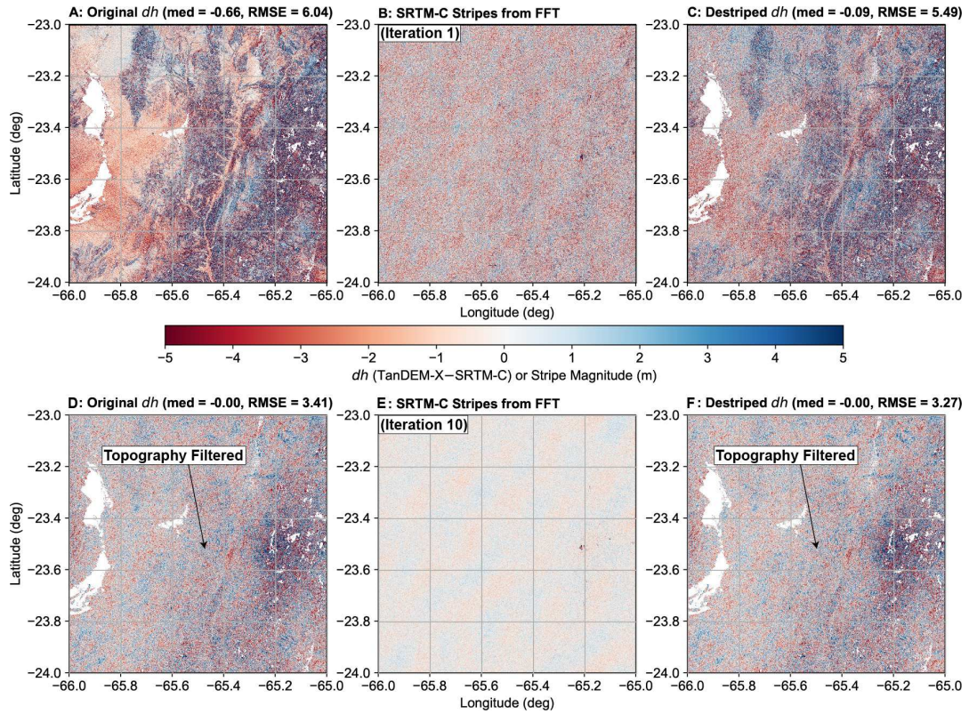
Figure A11 – Two iterations of more aggressive FFT destriping from one tile (S 24°, W 66°), same as in Figure 3.3. Top panel (A–C) show first iteration and bottom panel (D–F) show tenth iteration. We note that while the striping and remaining patches caused by SRTM-C collection biases are removed using the more aggressive approach, the true topographic noise is also filtered, which is not the aim of our correction steps.
