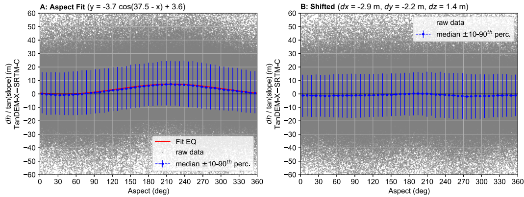
Figure 3.2 – Relationship of dh (normalized by tangent of slope) to aspect (A) before and (B) after co-registration and bilinear resampling of SRTM-C. We fit to equation 3.1 on all raw data. Note the close match between equation fit and median values. The cosine relationship in (A) is caused by overestimation of the SRTM-C on NE facing aspects (peaking at \sim 60^\circ ) and underestimation on SW facing aspects (peaking at \sim 220^\circ ). The resulting (dx, dy) shift vector is directed SW.
