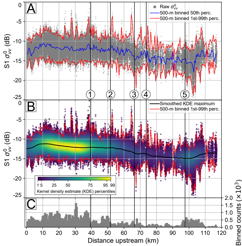
Figure 5.6 – Example point cloud and trendline extraction for one S1 scene (20180901). The tectono-geomorphic transitions (1–5) correspond to Figure 5.1B. (A) is the raw point cloud (masked for \text{NDVI} > 0.15 ), with the 50 th and 1 st –99 th percentile lines (binned in 500-m steps) plotted over it. To remove the spikiness and get an average trendline we go to (B), where the median line is replaced with the smoothed 2D KDE maximum. (C) shows the 15-m SAR pixel counts per 500-m bin. See Figure C1 in Appendix C for examples using TSX/TDX and ALOS2 scenes.
