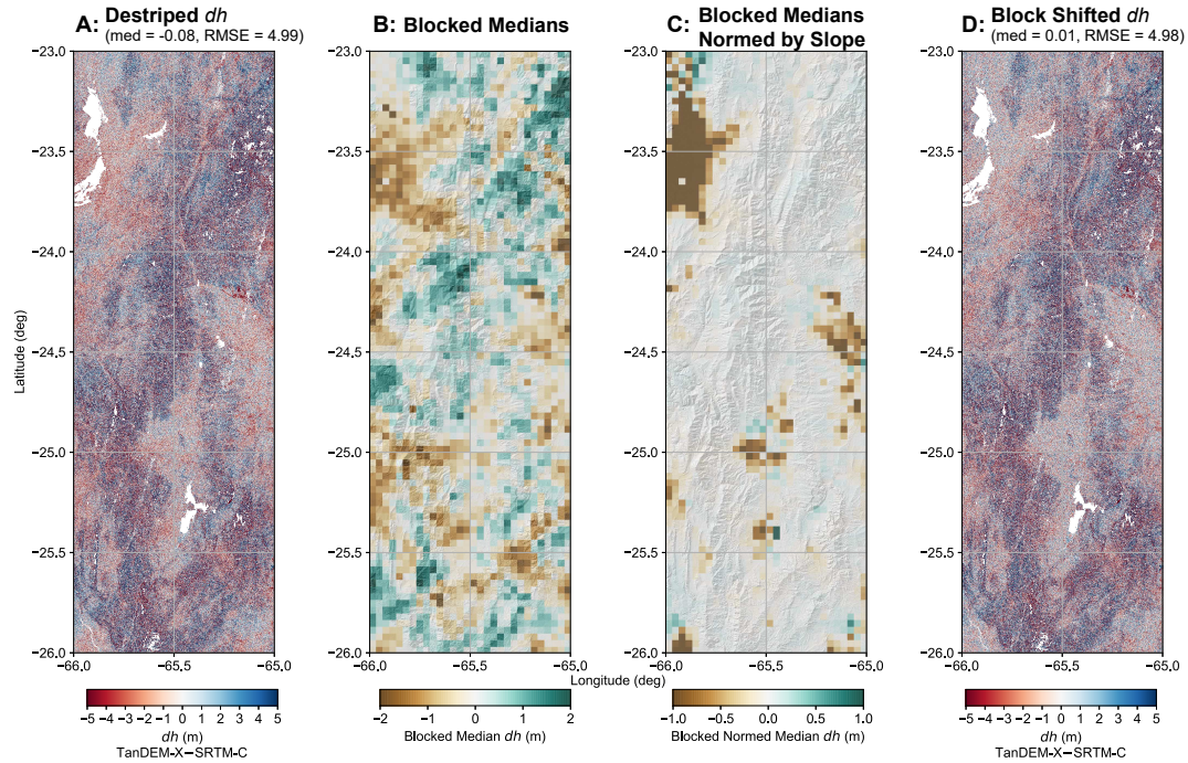
Figure 3.4 – Blocked shifting on three destriped and merged tiles (S 24–26°, W 66°). Blocks are 3.6 km in height and width. The (A) destriped median and RMSE both improve slightly in (D) the final shifted dh map. Note that the original blocked medians (B) show a slight pattern resembling the long-wavelength stripe bias from SRTM-C. In (C) we have normalized the median shifts by the median slope values, so as not to over-correct the steeper regions with higher uncertainties. The color scheme is changed for (B) and (C), and the scale of (C) is half the width of (B) since it only extends to the maximum allowable shift of \pm 1 m. Scales and color scheme in (A) and (D) are identical. Voids (white space) are untrustworthy pixels removed by TanDEM-X WAM cutoff prior to median calculation.
