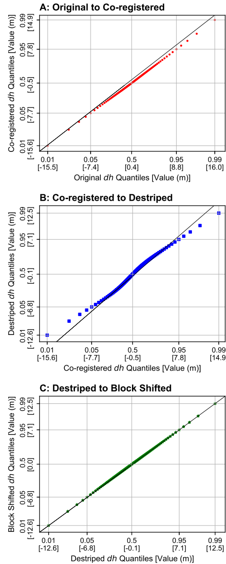
Figure 3.6 – Quantile-quantile (QQ) plots showing difference between each successive correction step from three tiles merged and processed (S 24–26°, W 66°). (A) original to co-registered, (B) co-registered to destriped, and (C) destriped to block shifted. We note that co-registration and destriping have the greatest effect on zero-median-shifting and narrowing the outliers. The quantiles (0.01, 0.05, 0.5, 0.95, and 0.99) and their respective values are indicated on each axis to highlight this effect.
