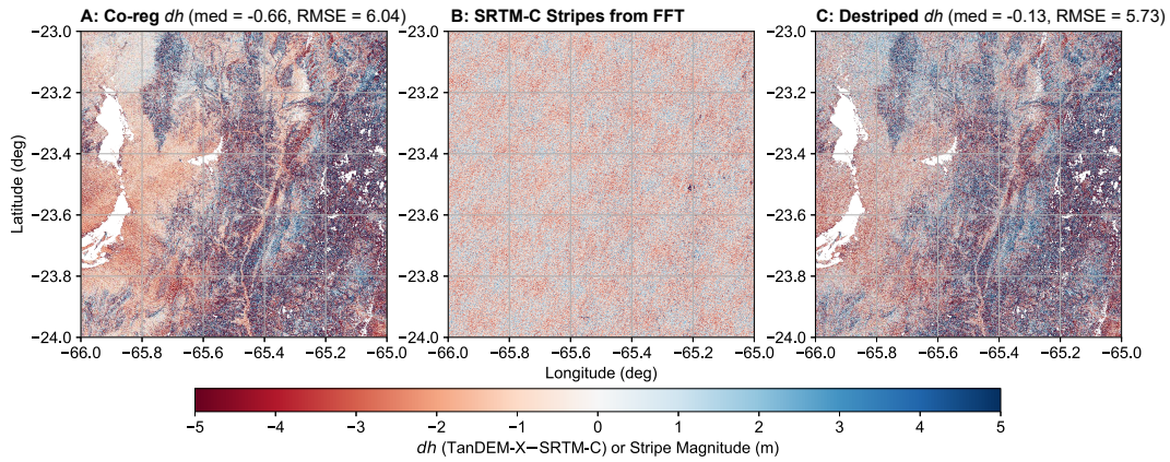
Figure 3.3 – One iteration of FFT destriping from one tile (S 24°, W 66°). Both median and RMSE improve from (A) the co-registered map to (C) the destriped map. Stripes removed by FFT are shown in (B). Note that (C) is not the final corrected map as iteration was run twice more before RMSE began to converge at 5% tolerance level. Voids (white space) are untrustworthy pixels removed by TanDEM-X WAM cutoff prior to destriping.
