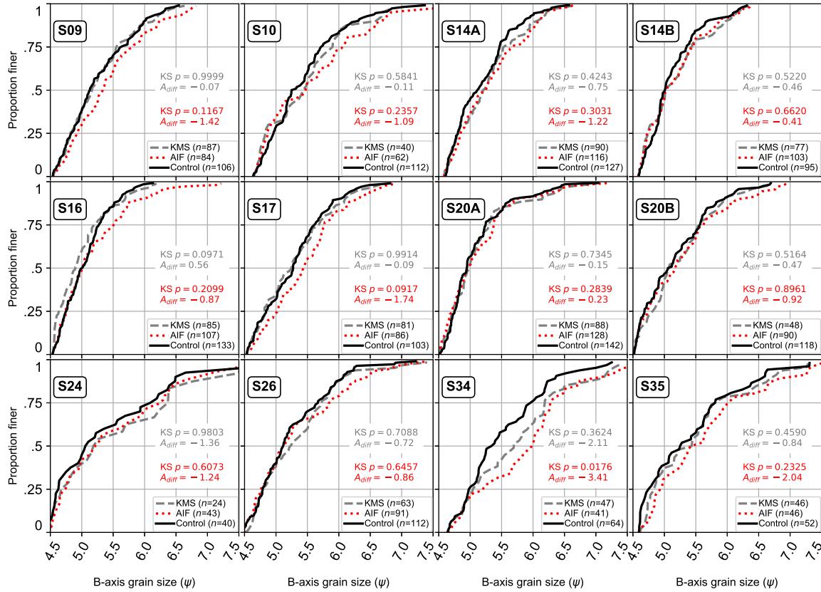
Figure B7 – Comparison of 20-pixel truncated grain-size distributions between hand-clicked control (black line), KMS PebbleCounts (gray, dashed line), and AIF PebbleCountsAuto (red, dotted line) for the 12 \times \sim 1.16 mm/pixel control sites. In corresponding colors are the p -value results of a KS-test and the A_{diff} approximate integral between the curves for each approach versus the control data. The legend indicates the number of grains ( n ) making up each curve. See Figure 4.6b in Chapter 4 for sites.
